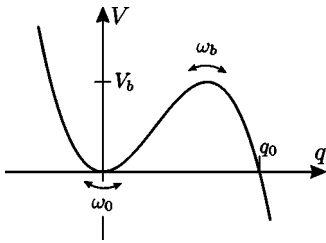
FIG. 3. Cubic potential as defined in Eq. (40).
