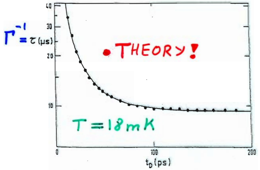
TUNNELING IN A JOSEPHSON JUNCTION SUBJECTED TO MEMORY FRICTION [Esteve et al. (79)]
