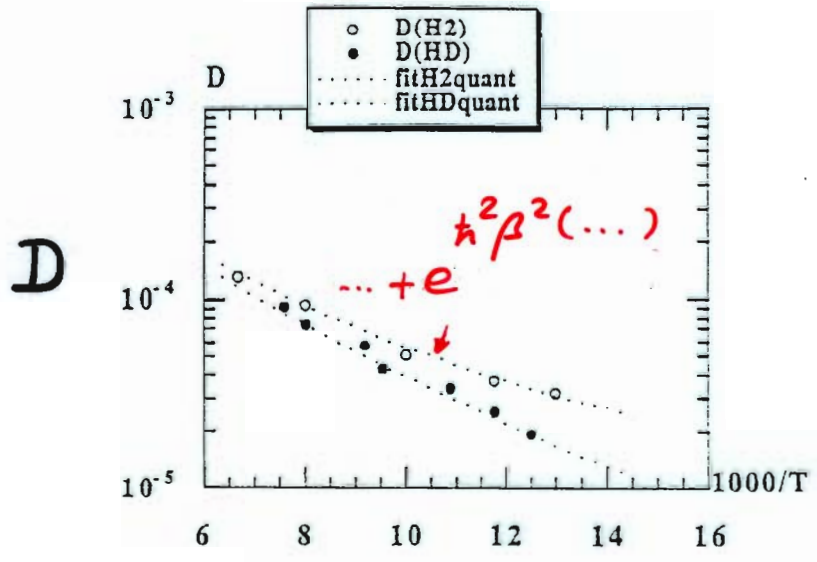
H 2 & HD sorbed in zeolites [Bouchand et al. (82)]
