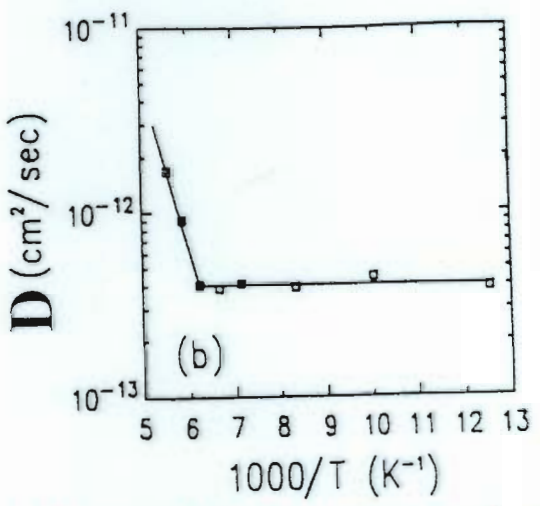
H on (110) tungsten [GOMER(82)]
