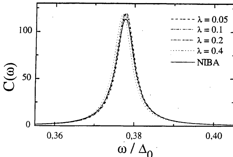
Fig. 2. Exemplary correlation function for a super-Ohmic bath ( s = 2 , K = 40 , \omega_c = 80 ). The different curves are obtained by using Eq. (13) for various values of \ell_0 = (2\lambda\Delta_r)^{-2} . The scale is set by \Delta_0 = 1 . For comparison the NIBA-curve is also shown. The maximum of the NIBA-curve is slightly shifted with respect to the flow equations and has been suitably rescaled in order to identify the peaks.
