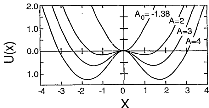
FIG. 1. The potential, showing a monostable initial state for A_0 = -1.38 and the switched bistable states at the values of A indicated.
