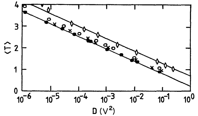
FIG. 6. \langle T \rangle in ms vs D in \text{V}^2 for A_0=-1.38 and A=3.0 . The values of \tau are 0.1, \bullet ; 0.5, \times ; 1.0, \circ ; and 4.9, \diamond . The solid lines are fits to the data.
