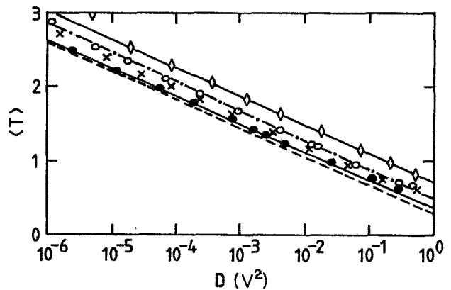
FIG. 7. \langle T \rangle in ms vs D in \text{V}^2 for A_0=-2.40 and A=4.0 . The values of \tau are 0.1, \bullet ; 0.5, \times ; 1.0, \circ ; and 5.0, \diamond . The solid lines are fits to the data. The dot-dashed and dashed lines are theoretical predictions for \tau=1.0 and 0.1, respectively.
