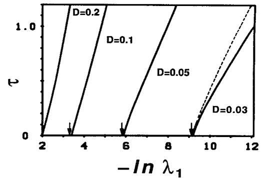
FIG. 1. First nonvanishing eigenvalue \lambda_1(\tau) of the non-equilibrium bistable flow in (1) as a function of noise color \tau . For D < 0.1 one finds the behavior in (2) with \alpha \approx 0.10 (see inset of Fig. 2). The arrows indicate the result (3) of the steepest-descent approximation at \tau=0 . The bridging result by Luciani and Verga (Ref. 20), i.e.,
