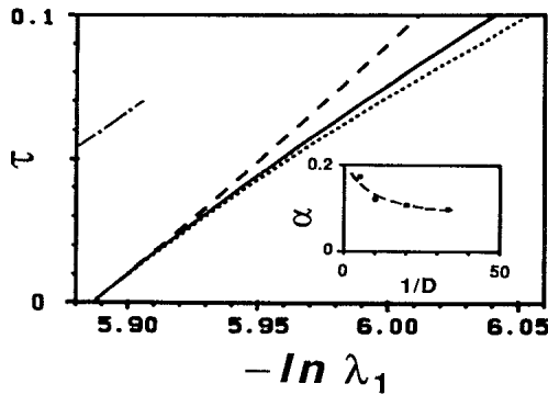
FIG. 2. The asymptotic behavior of \lambda_1(\tau) for vanishing noise color at D=0.05 . Solid line, numerical result; dashed line, \lambda_1^{\text{EFP}}(\tau) from Ref. 8; dotted line, \lambda_1^{\text{EFP}}(\tau) from Ref. 6; dash-dotted line, steepest-descent prediction \lambda_1(\tau) = (\sqrt{2}/\pi)(1 - 1.5\tau)\exp(-1/4D) .
