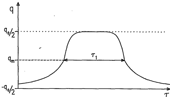
FIG. 5. A sketch of a bouncelike trajectory (3.10), for a general value of \tau_1 , given by Eq. (3.11).
