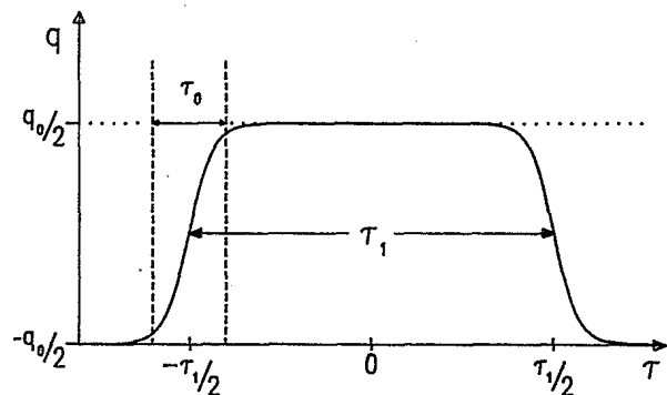
FIG. 2. A bounce trajectory. The instanton and anti-instanton parts of the trajectory have typical widths \tau_0 and are located at -\tau_1/2 and +\tau_1/2 , respectively.
