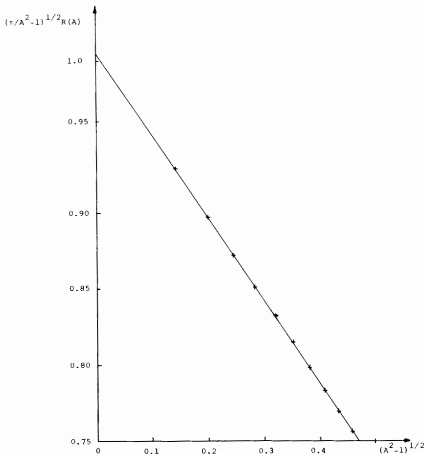
Fig. 4. (—) Scaling function R(A) in (3.25) versus (A^2 - 1)^{1/2} compared against (x) the numerical results.
