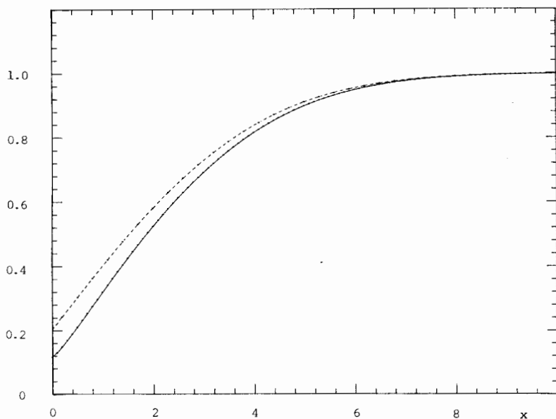
Fig. 5. (—) Numerical solution of the scaled boundary layer function (3.14), h(x) , and (---) the extrapolated asymptotic curve (3.32), h^{as}(x) , for the same value of A = 1.025 .
