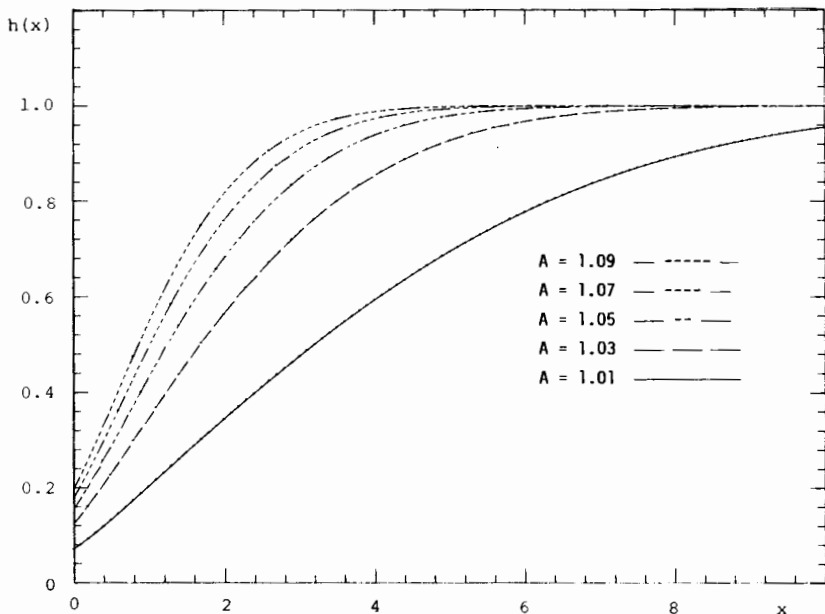
Fig. 3. Numerical solution of the scaled boundary layer function (3.14), (3.15) for various A values [see (3.14b)].
