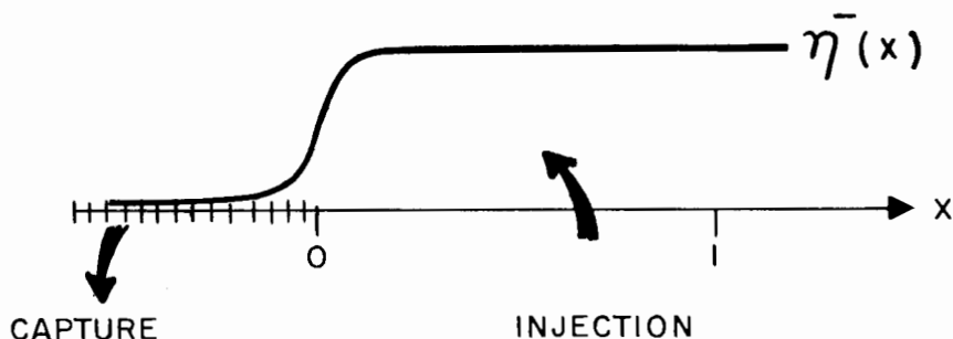
Fig. 6. Typical behavior of the form function \eta^-(x) describing the deviation from the equilibrium invariant probability. It changes drastically within the boundary layer width (2\epsilon)^{1/2} .
