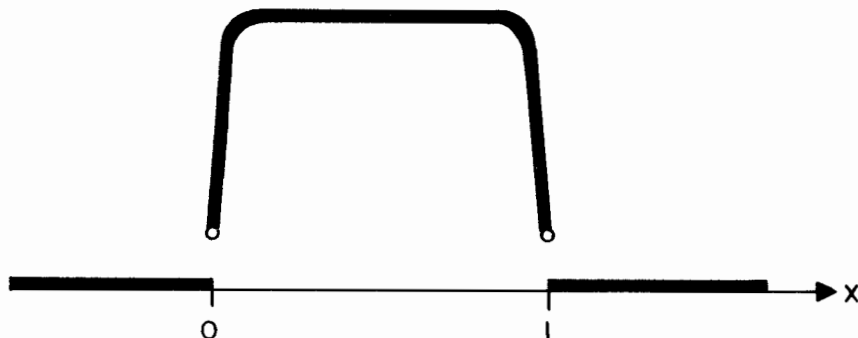
Fig. 2. Qualitative sketch of the MFPT t(x) , (3.4), versus x . Illustrated are the absorbing lines outside the domain of attraction, as well as the typical boundary jumps at the exit points.
