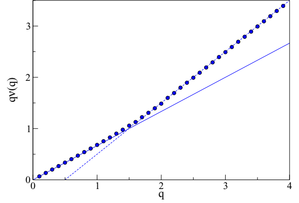
FIG. 6. (Color online) The spectrum of exponents qv(q) versus q exhibits piecewise linear behavior. The finite-time simulations (dots, parameters as in Fig. 5), for the uniform model, perfectly agree with theory (lines): for q < \alpha qv(q) = q/\alpha otherwise qv(q) = q + 1 - \alpha [see Eq. (76)]. Here \alpha = 3/2 .
