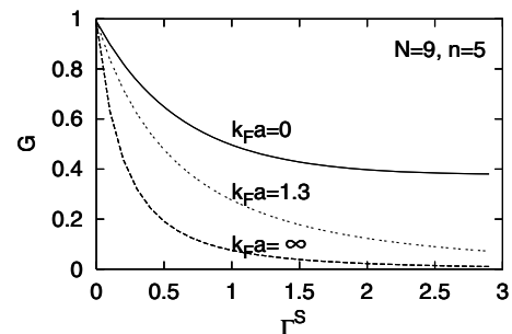
Fig. 6. Decay of the conductance oscillation with the wire-substrate coupling strength \Gamma^S for a substrate with delocalized electrons ( k_Fa = \infty ), with localized electrons ( k_Fa = 0 ) and for k_Fa = 1.3 . The other parameters are N = 9 , n = 5 , and \varepsilon_0 = 0 .
