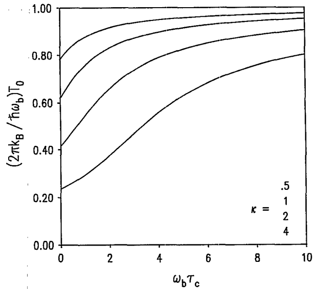
FIG. 2. Same as Fig. 1 for model B. The crossover temperature is depicted as a function of the dimensionless memory time \omega_b\tau_c for various values of the noise strength \kappa = \gamma/\omega_b .
