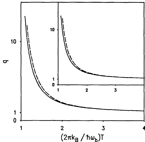
FIG. 3. The approximation (16) for the quantum correction factor q (dashed line) compared with the exact result (solid line) for model A, with parameters \omega_b = \omega_0 , \kappa = 0.5 , and r = 0.25 . The inset shows the same quantities for model B, with parameters \omega_b = \omega_0 , \kappa = 0.5 , and \omega_b \tau_c = 0.5 .
