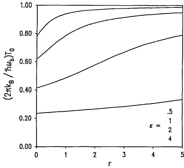
FIG. 1. The dimensionless crossover temperature (2\pi k_B/\hbar\omega_b)T_0 = \omega_R/\omega_b for model A depicted as a function of the mass ratio r for various values of the dimensionless noise strength \kappa = \gamma_0/\omega_b .
