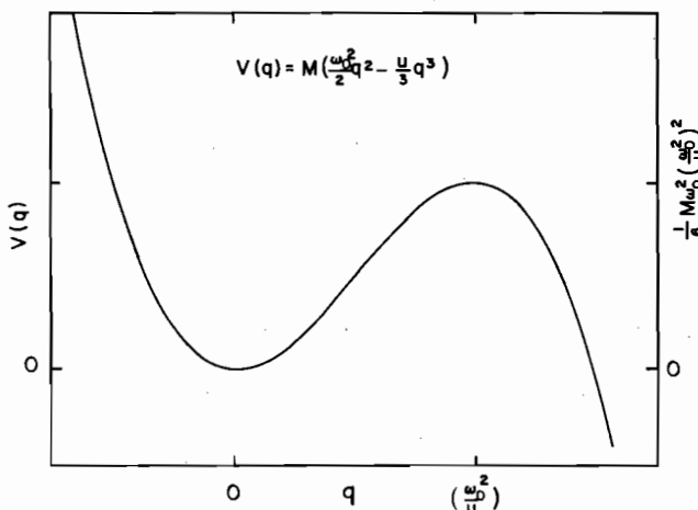
FIG. 1. The metastable potential well V(q) = M[(\omega_0^2/2)q^2 - (u/3)q^3] . The top of the potential barrier is located at q = \omega_0^2/u .
