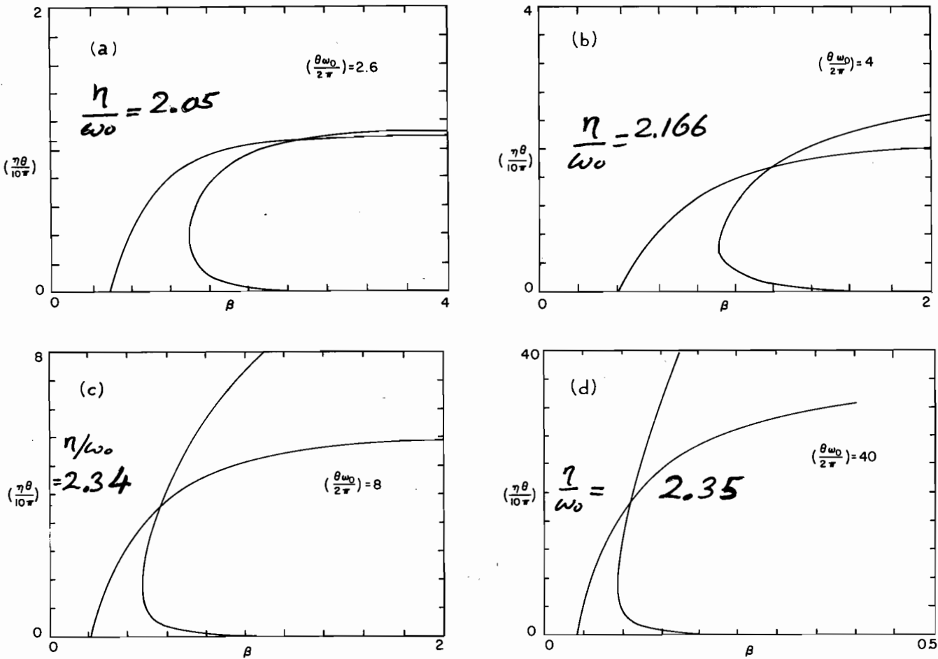
FIG. 2. The graphical solutions of the two coupled quadratic equations (3.3) for a sequence of decreasing temperatures. The intersection of the two curves defines (\eta\theta/10\pi) and \beta .
