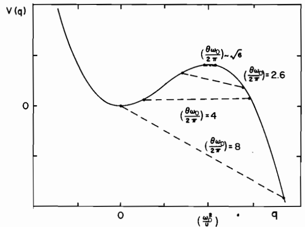
FIG. 4. The variation of the extrema of the bounce trajectories as the temperature is decreased. At T_0 , the crossover temperature, the bounce trajectory remains at the top of the potential barrier. As T is decreased the bounce exists over a finite spatial region. The spatial extent saturates at T=0 .
