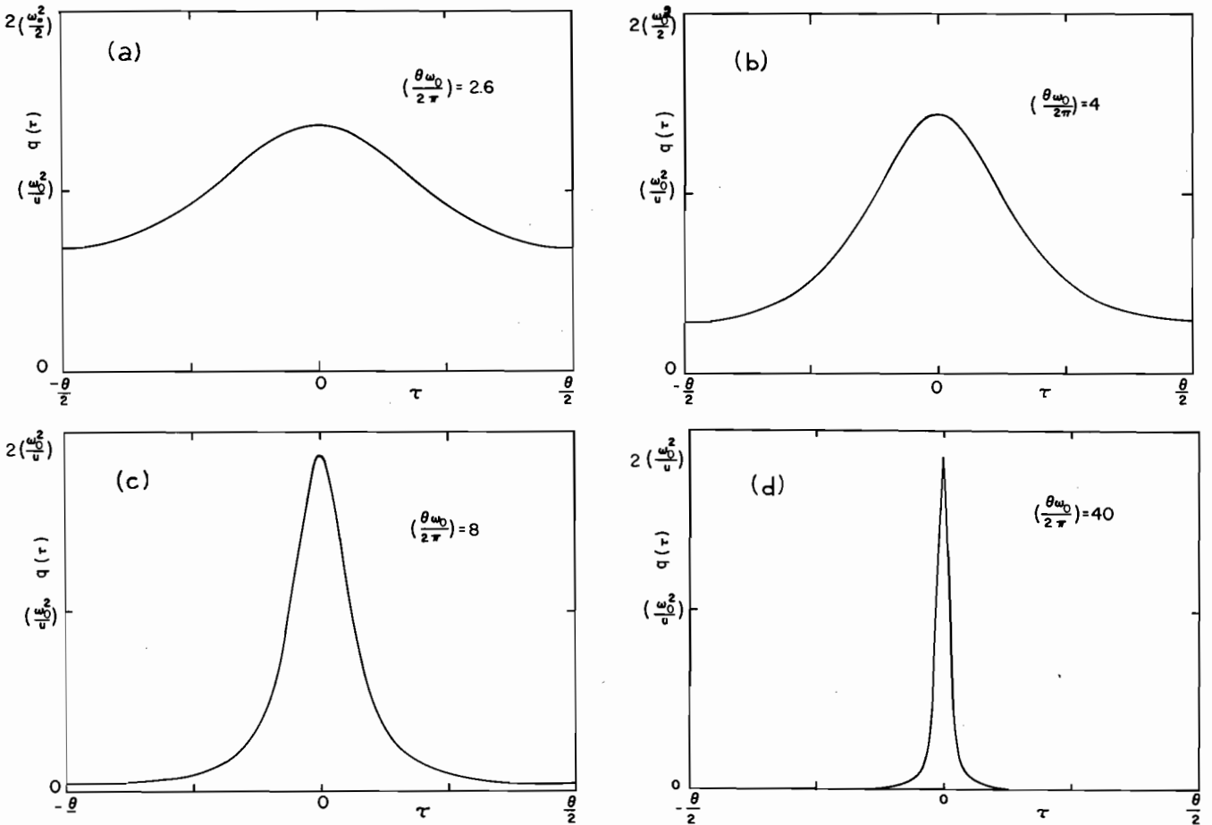
FIG. 3. The bounce trajectories corresponding to the same sequence of decreasing temperatures depicted in Fig. 2.
