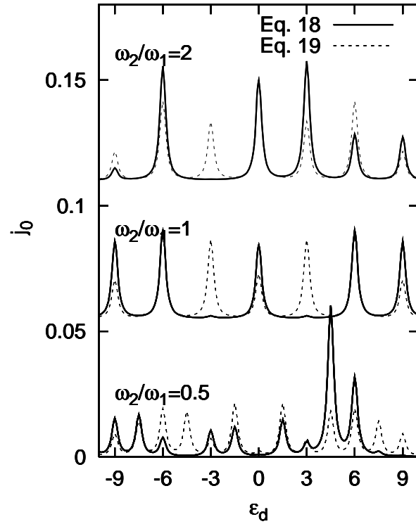
Fig. 4. Dc-current as a function of \varepsilon_d obtained for commensurate frequency ratios \omega_2/\omega_1 = 2, 1 , and 0.5 according to Eq. 17 with the transmission given by Eq. 18 (solid lines) and for a slightly off-commensurate frequency; i.e., \omega_1 = 3, \omega_2 = 5.999 , see Eq. 19 (broken lines). All parameters are the same as in Fig. 3
