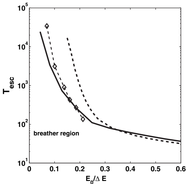
Fig. 5: Mean escape time T_{esc} vs. the ratio of energy per unit and barrier energy, i.e. E_0/\Delta E for the noise-free case k=0 mode (solid line), randomized initial conditions (diamonds) and noise-assisted case (dashed line), respectively. The parameters are: q_0=0.40 , \Delta q=0.1 , \omega_0^2=2 , a=1 , \kappa=0.3 and \gamma=0.1 , N=100 .
