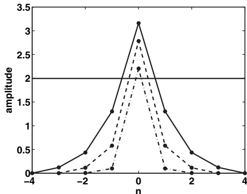
Fig. 3: The amplitude profile is depicted for a critical chain configuration, being symmetrically centered at n = 0 , for different coupling strengths: \kappa = 0.1 (dash-dotted line), \kappa = 0.5 (dashed line), and \kappa = 1 (solid line). Note that for better illustration only a small part of the lattice chain with sizeable elongations is shown. The chosen parameters are \omega_0^2 = 2 , a = 1 for a chain with N = 100 .
