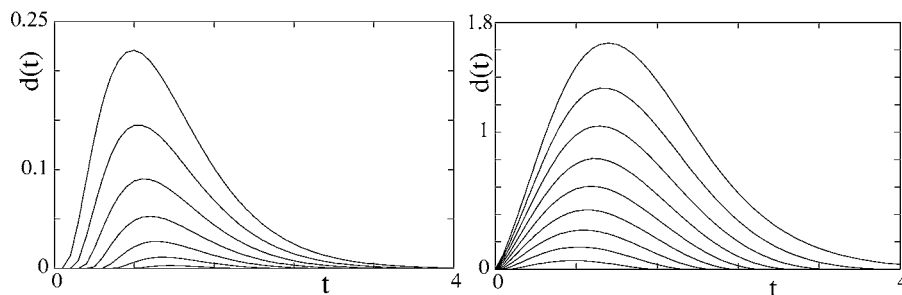
FIG. 4. Time evolution of the bimodality depth originating from a sudden drop of temperature. The system evolves from p(x,0)=p_{st}(x) for the initial temperature T=T_i to the final stationary state p_{st}(x) with temperature T=T_f . Assumed value of D=0.1T . The left panel shows results obtained for the Ginzburg-Landau model with T_i=10, T_f=1.3 , and \alpha=0.1 . Here, the curves from top to bottom correspond to \epsilon=\epsilon_0(T-1) with \epsilon_0=0.02, 0.04, \dots, 0.14 . The right panel shows results obtained for the Josephson junction model with T_i=10 and T_f=0.1 . The curves from the top to the bottom correspond to \epsilon=0, 0.1, \dots, 0.8 .
