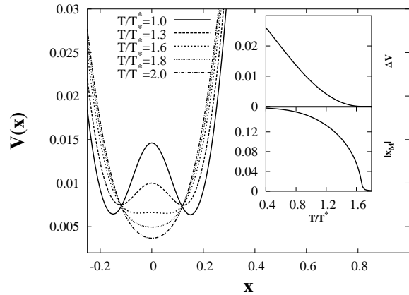
Fig. 1. The generalized potential V(x, t) \equiv V(x) defined by Eq. (4) is depicted in the absence of the external driving, i.e. when \lambda(t) = 0 for selected values of the scaled temperature T/T^* . Upper inset: The corresponding barrier height \Delta V of the potential as a function of temperature. Lower inset: The position of the minimum x_M of the corresponding potential as a function of temperature.
