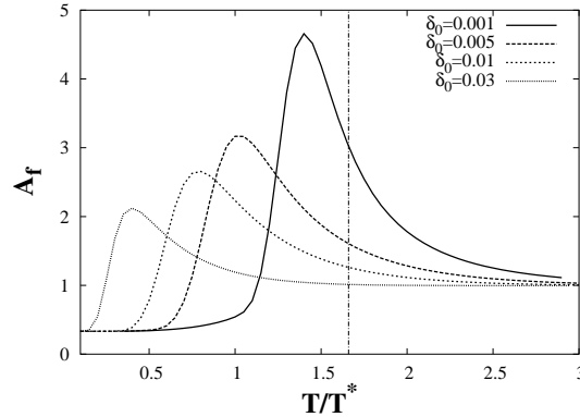
Fig. 2. The amplification factor (see in text and in Ref. [25]) is depicted vs. the scaled temperature for several values of the noise intensity \delta_0 and a fixed driving strength a_0 = 0.01 . The vertical line depicts the critical temperature above which the generalized potential V(x) in Fig. 1 becomes monostable.
