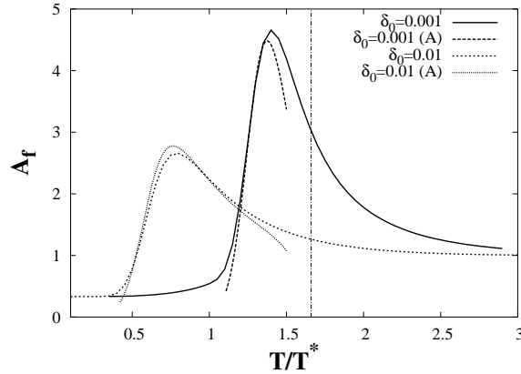
Fig. 3. The comparison of the Stochastic Resonance as quantified by the amplification factor between the numerical data with the analytic linear response formula (10), labeled by A.
