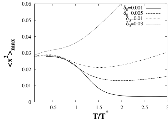
Fig. 4. Amplitude of the re-scaled mean magnetic energy \langle x^2(t) \rangle vs. the temperature for several values of the noise strength \delta_0 .
