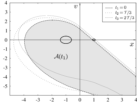
Fig. 2 Phase space diagram for a typical metastable potential with additive sinusoidal driving (3), namely the piecewise parabolic potential (75) with \bar{x}_s = \omega_u^2 = -1 , \bar{x}_u = \omega_s^2 = m = \Delta V = \Omega = 1 , \eta = 0.5 , A = 0.2 . Solid line: Stable (left) and unstable (right) periodic orbit. Dashed lines: Separatrix at different times t_1 = 0 , t_2 = T/3 , and t_3 = 2T/3 . Grey area: Domain of attraction \mathcal{A}(t_1) of stable periodic orbit x_s(t) at time t_1 .
