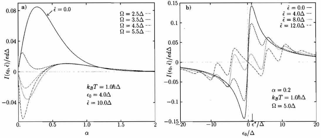
Fig. 2. – Dimensionless time-averaged current I(ed\Delta) plotted vs. the dissipative Ohmic strength \alpha (fig. 2a) and vs. the dc-bias \epsilon_0 (fig. 2b)). For weak dissipation a negative current, which is maximal for an optimal value of \alpha is found. For stronger dissipation the current becomes independent of the ac-frequency and on dissipation on a wide range.
