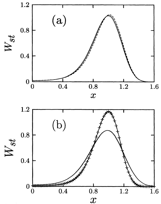
FIG. 1. (a) The stationary probability density for positive-valued x , W_{st}(x; \tau) = W_{st}(-x; \tau) , is shown for white and colored noise strengths D=Q=0.05 . The correlation time of the colored noise is \tau=1 . The solid line gives the numerical (MCF) result, the dashed line represents the small- \tau theory, while the dotted line depicts the crossover approximation which essentially agrees with the large- \tau approximation. (b) The same as in (a) for different correlation times: The results with \tau=10 are depicted by crosses for the crossover approximation and as a solid line for the numerical (MCF) results. The results of the large- \tau approximation in (6) agree within line thickness with the numerical results for \tau=10 . The other set of lines shows the results for \tau=0.1 : The numerical results (solid) and the crossover approximation (dotted); here, the small- \tau theory in (4) agrees almost within line thickness with the numerical results.
