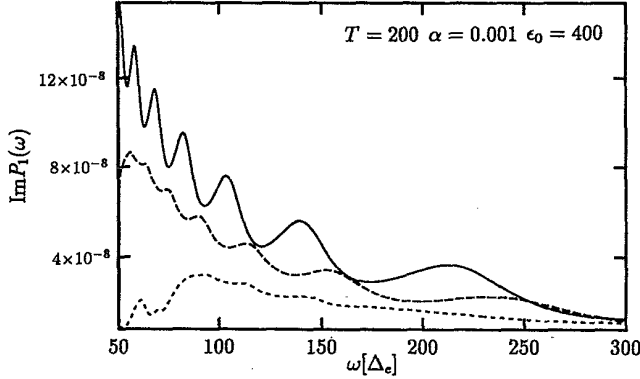
FIG. 2. Same plot with same values for \alpha , T , and \epsilon_0 as in Fig. 1, but with different values of the driving amplitude, \hat{\epsilon} = 400\Delta , 600\Delta , and 1000\Delta (full, dashed, and dotted line, respectively).
