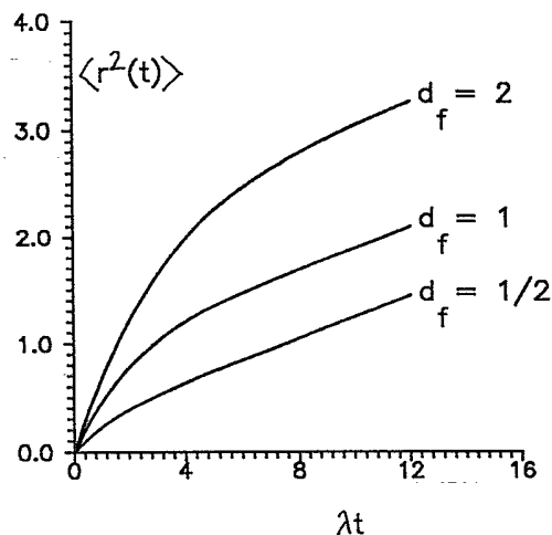
FIG. 5. Same as in Fig. 4 but for the fixed quotient of death to birth rates \mu/\lambda=0.1 (weak detachment of particles from the cluster), 6D_0/\lambda M_0^\beta=1 , and three values of the cluster dimension d_f=1/2, 1, 2 .
