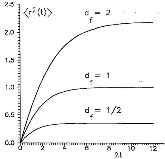
FIG. 7. The mean square displacement (41) of the cluster mass center as a function of rescaled time \lambda t for the pure birth growth model ( \mu=0 ) with a linear birth rate and 6D_0/\lambda M_0^\beta=1 . If t \rightarrow \infty then all curves tend to constant values (saturation).
