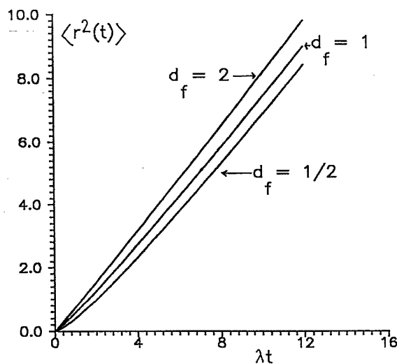
FIG. 6. Same as in Fig. 5 but for the strong detachment of particles from the cluster, \mu/\lambda=0.8 .
