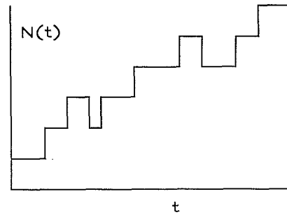
FIG. 3. Sketch of a possible realization of the linear birth-and-death process N(t) with the initial value N(0)=1 , probabilistic rates \lambda > \mu > 0 , and unit up and down steps N(t_{i+1}) - N(t_i) = \pm 1 .
