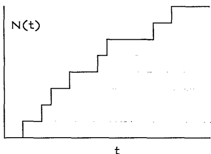
FIG. 1. Sketch of a possible realization of the Poisson process N(t) with the initial value N(0) = 0 and unit steps at random instants t_i, i = 0, 1, 2, \dots, N(t_{i+1}) - N(t_i) = 1 .
