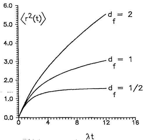
FIG. 2. The mean square displacement (17) of the cluster mass center for the Poisson growth model as a function of rescaled time \lambda t and for three selected values of the cluster dimension d_f = \frac{1}{2}, 1, 2 . The remaining parameters are fixed in such a way that 6D_0/\lambda M_0^\beta = 1 .
