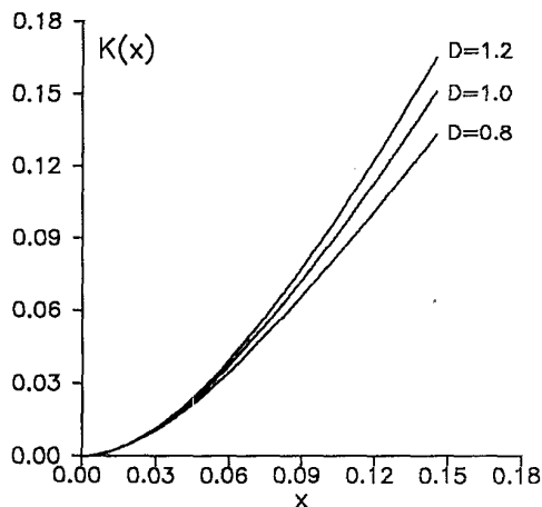
FIG. 2. The diffusion function K(x) for a=4\alpha , \alpha=1 , i.e., \nu=-\frac{1}{2} , and various values of the noise intensity D : the small- x case. For fixed \nu=-2\alpha/a , K(x) depends linearly on \alpha .
