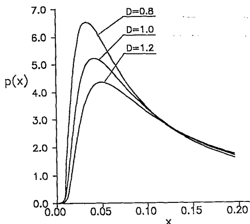
FIG. 1. Some selected examples of the stationary probability distribution (8) for a=4\alpha are depicted at various values of the noise intensity D .
