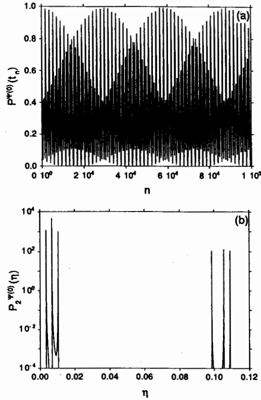
Fig. 1. Driven tunneling at the fundamental resonance \omega = E_3 - E_2 . (a) Time evolution of P^{\Psi(t_0)}(t_n) over the first 10^5 time steps; (b) local spectral two-point correlation function P_2^{\Psi(t_0)}(\eta) obtained from (a). The parameter values are D = 2 , S = 2 \cdot 10^{-3} , and \omega = 0.876034 .
