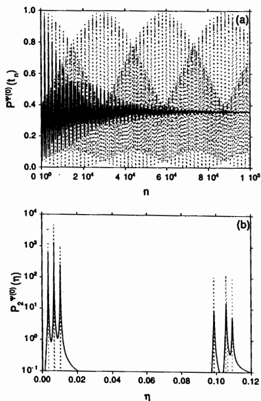
Fig. 3. Driven tunneling with dissipation. (a) Time evolution of P^{\Psi(0)}(t_n) over the first 10^5 time steps; (b) local spectral two-point correlation function P_2^{\Psi(0)}(\eta) obtained from (a). The parameter values are as in the corresponding conservative case shown in Fig. 1 (repeated here as dashed lines), but with a finite damping constant, \gamma = 4 \cdot 10^{-5} , at T = 0 .
