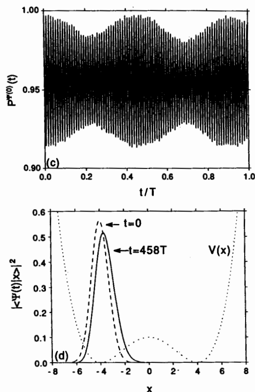
Fig. 2. Coherent suppression of tunneling at an exact crossing \epsilon_{2,-1} = \epsilon_{1,1} . (a) One of the manifolds in the (S, \omega) -plane where this crossing occurs (data obtained by diagonalization of the full Floquet operator for the driven double well are indicated by crosses, the full line has been derived from a two-state approximation, the arrow indicates the parameter point for which the subsequent parts of the figure have been obtained); (b) time evolution of P^{\Psi(0)}(t_n) over the first 10^3 time steps; (c) time evolution of P^{\Psi(0)}(t) within the first period of the driving; (d) |\langle \Psi(t_n) | x \rangle|^2 at n = 458 (dashed line), compared with the initial state (full line) (the dotted line indicates the unperturbed potential). The parameter values are D = 3 , S = 3.171 \cdot 10^{-3} , and \omega = 0.01 , that is, \omega = 52.77\Delta .
