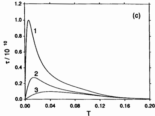
Fig. 5. Coherent suppression of tunneling in the presence of dissipation. (a) Time evolution of the autocorrelation function P^{\sigma(0)}(t_n) , over the first 10^7 time steps, at a parameter point ( D = 2 , S = 3.171 \cdot 10^{-3} , and \omega = 0.01 ) close to a manifold where the tunnel splitting vanishes, for \gamma = 10^{-6} , a cutoff frequency \omega_c = 1 , and various values of T , starting from a coherent state centered in one of the wells; (b) the first 2 \cdot 10^4 time steps from (a) on an enlarged time scale; (c) temperature dependence of the decay time \tau of P^{\sigma(0)}(t_n) (defined by P^{\sigma(0)}(t_n) \approx \exp(-n/\tau) ) for three values of the detuning \Delta\omega = \omega - \omega_{loc}(S) from the localization manifold (graph 1: \Delta\omega = -1.4 \cdot 10^{-7} , as in part (a), 2: \Delta\omega = 5.0 \cdot 10^{-7} at S = 3.1712 \cdot 10^{-3} , 3: \Delta\omega = 1.4 \cdot 10^{-6} at S = 3.1715 \cdot 10^{-3} ). The other parameters are as in part (a). The data shown do not extend down to T = 0 , where \tau(T) diverges, but start only with the rising part of this function.
