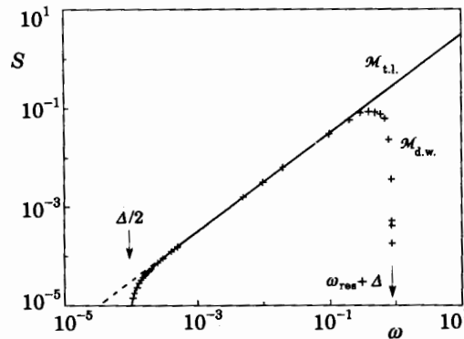
Fig. 1. - Double-logarithmic plot depicting the one-dimensional manifolds along which the first two quasi-energies cross for the first time: \mathcal{M}_{d.w.} (double well) and \mathcal{M}_{t.l.} (two level). The dashed line has been evaluated from the first zero of the Bessel function J_0(2b/\omega) , see (17). The D -parameter used is D = 2 , i.e. \Delta = 1.895 \cdot 10^{-4} .
