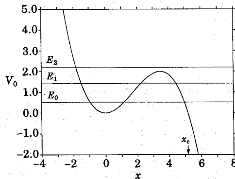
Fig. 1. – Unperturbed ( S = 0 ) metastable potential V_0(x) of the Hamiltonian in eq. (1) with D = 2 , supporting two quasi-stationary states under the barrier. The horizontal lines indicate the positions of the real parts of the resonance energies E_0 , E_1 , E_2 .
