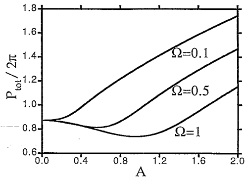
FIG. 6. The total “power” P_{\text{tot}} , i.e., the integral over the spectral density (4.21), is depicted as a function of the driving amplitude A at D=0.1 for three different driving frequencies \Omega .
