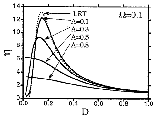
FIG. 2. The signal amplification factor \eta (3.13) is depicted as a function of the noise strength D at \Omega=0.1 for increasing values of the driving amplitude A . The result of LRT (4.15) is plotted as the dotted curve.
