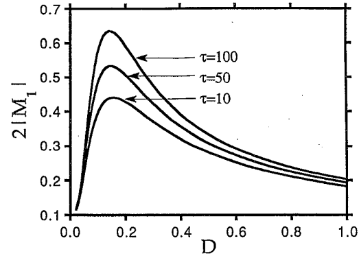
FIG. 4. The absolute value of the Fourier coefficient M_1 is plotted as a function of the noise strength D at \Omega=0.1 and A=0.2 for decreasing values of the coherence time \tau .
