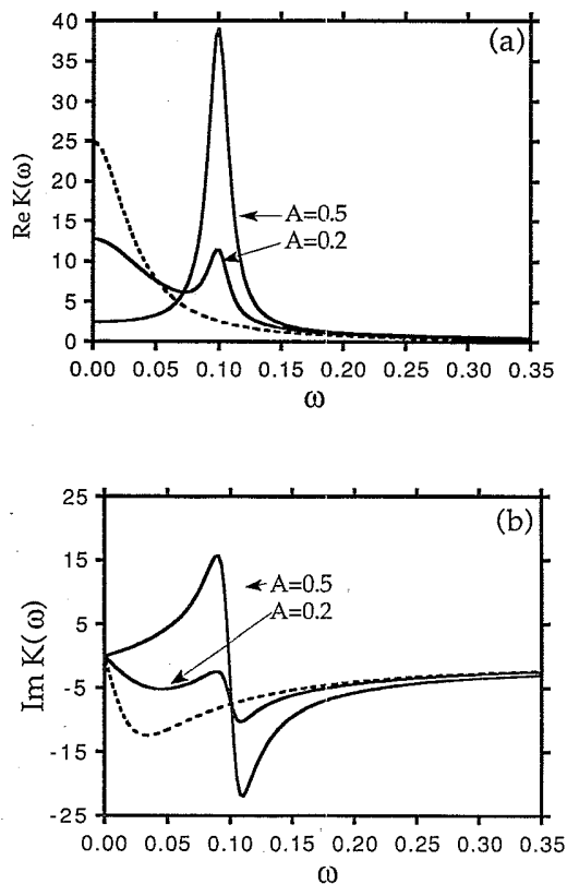
FIG. 5. The real part (a) and the imaginary part (b) of the one-sided Fourier transform of the correlation function K(\omega) (5.1) are shown at \Omega=0.1 zero driving amplitude (dotted lines) and for A=0.2 and 0.5 .
