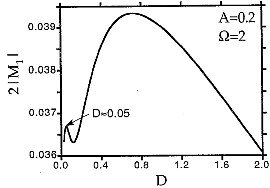
FIG. 3. The absolute value of the Fourier coefficient M_1 is shown as a function of the noise strength D at \Omega=2 and A=0.2 . The secondary resonance at D \approx 0.05 is indicated by an arrow. Note the self-similar shape of this secondary peak as compared with the main peak.
