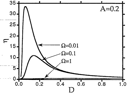
FIG. 1. The signal amplification factor \eta (3.13) is shown as a function of the noise strength D at A=0.2 for three different driving frequencies \Omega .
