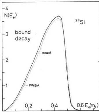
Fig. 2. The calculated energy spectrum N(E_e) for bound muon decay in ^{28}\text{Si} is plotted versus the total energy E_e given in units of the free muon rest mass. The solid line shows the exact spectrum calculated with eq. (9), whereas the dotted line shows N(E_e) in the PWBA.
