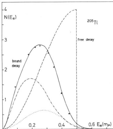
Fig. 1. The calculated electron spectra N(E_e) for bound muon decay in ^{205}_{81}\text{Tl} is plotted for various approximations versus the total energy E_e of the electron in the CM system of the muonic atom. The dotted line shows N(E_e) in the PWBA, the dashed-dotted line gives the spectrum calculated with distorted electron wave functions, and the solid line shows the spectrum evaluated by means of eq. (9). The crosses correspond to calculations of Huff [4] but for the charge number Z = 82 . The free muon decay is included for comparison. The energy of the electron is given in units of the free muon rest mass.
