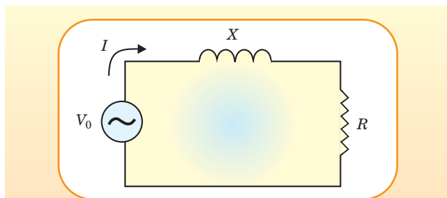
Figure 5. A model circuit. An AC voltage source V_0 generating a current I through a resistance R and inductor X models important features of transmission in the electric power grid.
