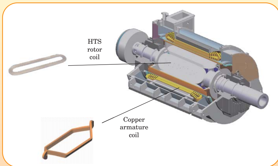
Figure 4. Rotating machines.
