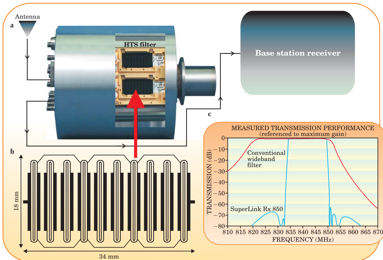
Figure 7. Improved wireless communication. Some 4000 HTS filters are currently in use at wireless base stations in the US. (a) The filters (black) sit in a cryogenic chamber between the station's antenna and receiver. (b) The filter shown incorporates 10 folded, weakly coupled HTS strips. (c) A plot of signal transmission versus frequency demonstrates the enhanced selectivity of the HTS filter over that of a conventional normal-metal filter. (Courtesy of Superconducting Technologies Inc.)
