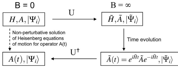
FIG. 1. The forward-backward transformation scheme induces a nonperturbative solution of the Heisenberg equations of motion for an operator. U denotes the full unitary transformation that relates the B=0 to the B=\infty basis (Ref. 15).
