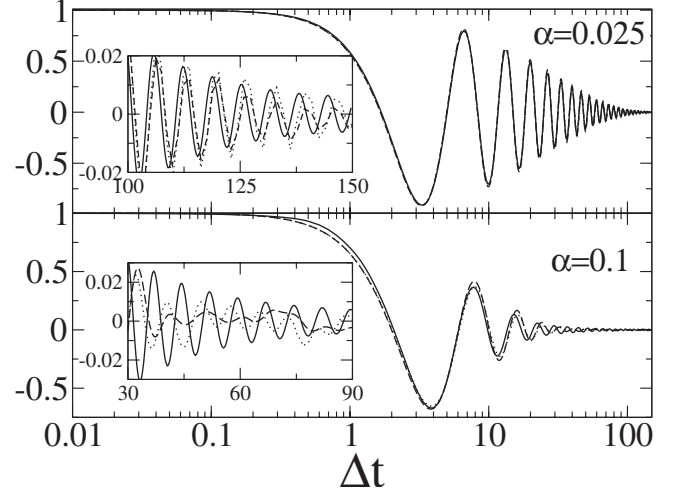
FIG. 2. Real time evolution of the spin expectation value \langle \sigma_z(t) \rangle starting from a polarized spin in the z direction with a relaxed Ohmic bath (see text) for two different values of \alpha and \omega_c/\Delta=10 . The full lines are the flow equation results, the dashed lines are TD-NRG curves for \Lambda=2.0 , and the dotted lines are for \Lambda=1.41 . The TD-NRG results are courtesy of Anders (see Ref. 11). The various curves agree extremely well except for very long times shown in the insets.
