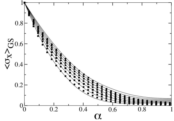
FIG. 3. Ground-state expectation value of \sigma_x . Comparison of flow equation results (curves) and NRG data (squares) from Ref. 19 for an Ohmic bath with damping \alpha . The results are for \omega_c/\Delta = 25, 28.6, 33.3, 40, 50, 66.7, 100 from top to bottom.
