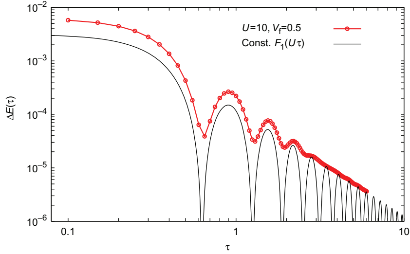
Figure 4. Excitation energy \Delta E(\tau) after the linear ramp (28a) of the hopping amplitude within the insulating phase ( U = 10 , V_i = 1 , V_f = 0.5 ), compared to equation (30) for small ramp amplitudes ( F_1 given by equation (29a)).
